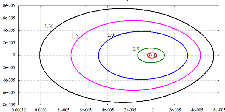
Fig. 2 Radial strains at the contact line in polar coordinates for kH = 0.1, 0.5, 1.0, 1.2, 1.38
